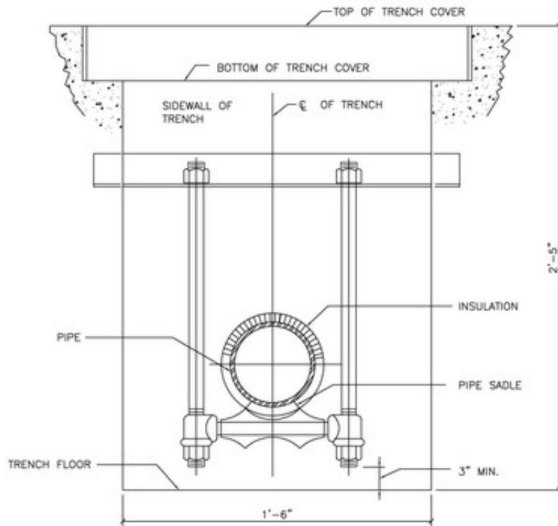
DETAIL FOR PIPE TRENCH
